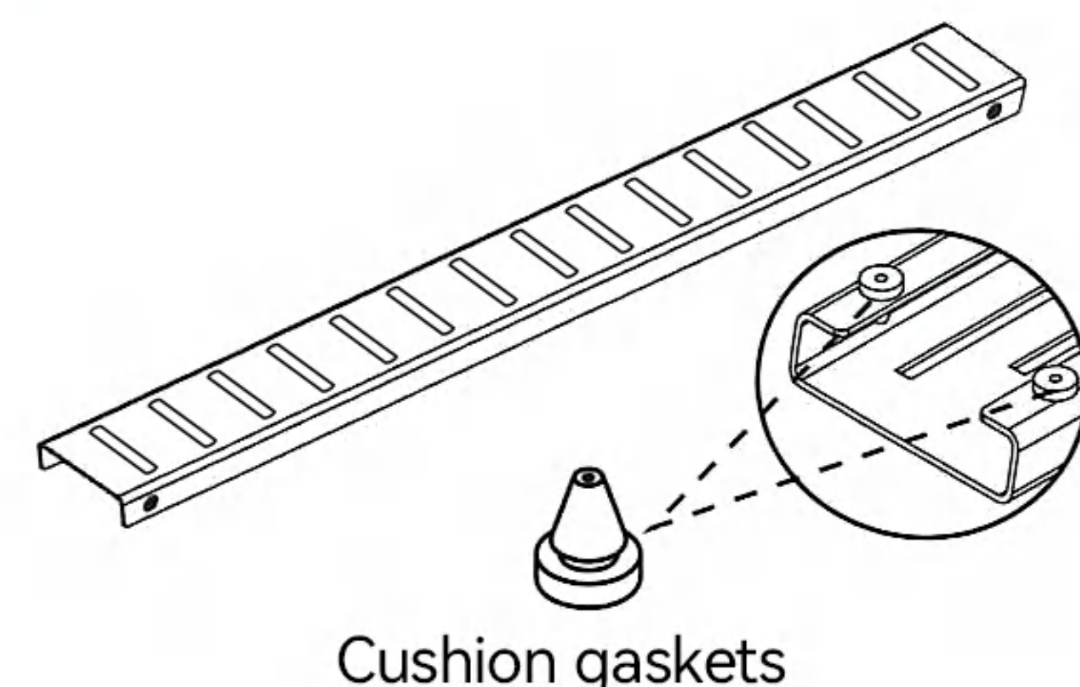
C. Decorative finish grating
