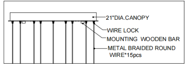
CANOPY DETAIL
