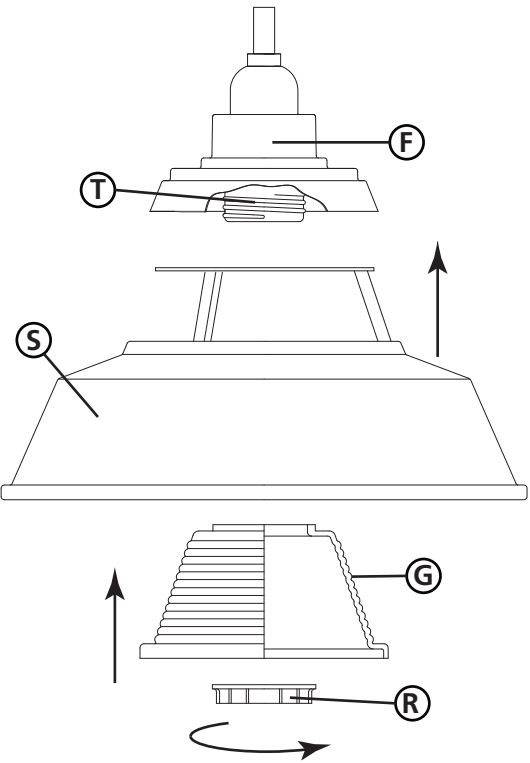
DRAWING 1 - GLASS INSTALLATION
