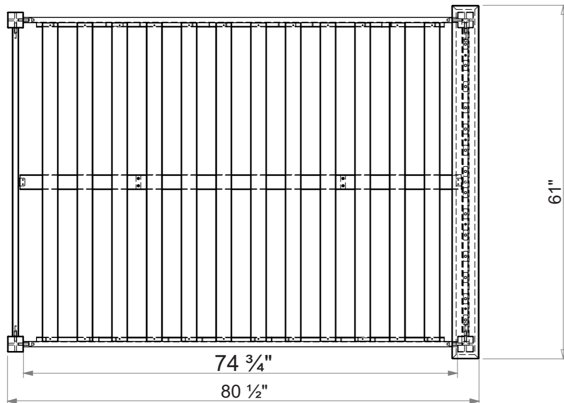
Top View
