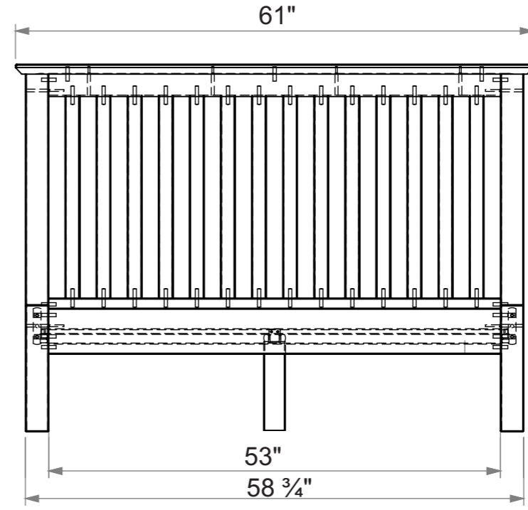
Frontal View
