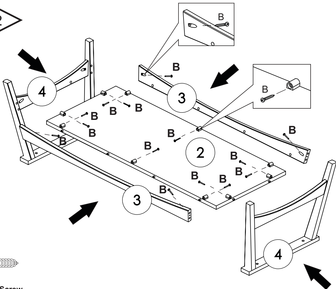
B - 4,0 x 35 Screw Qty. 14
