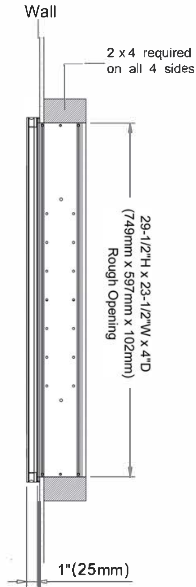
Recessed Mount
