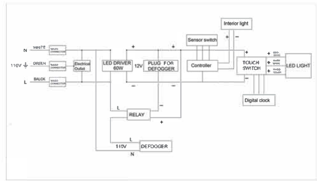
Circuit Diagram
