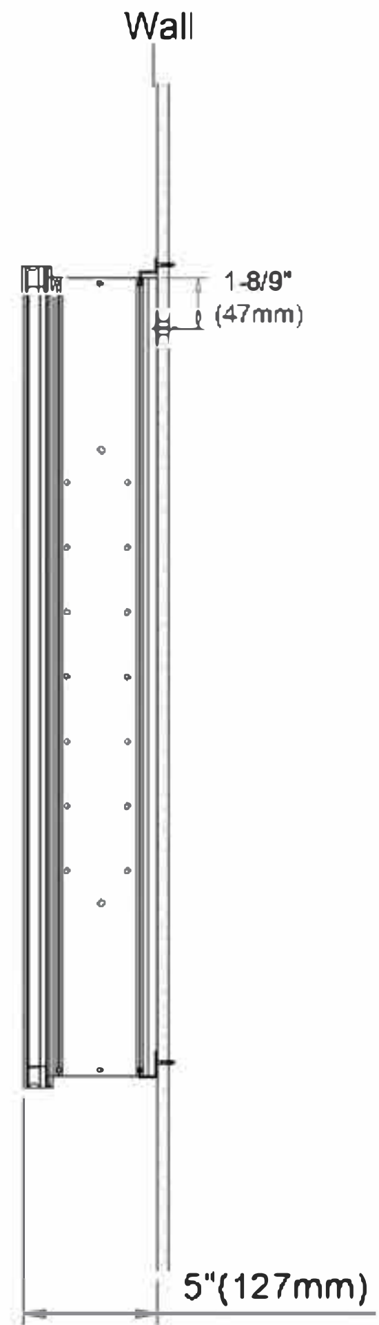
Surface Mount
