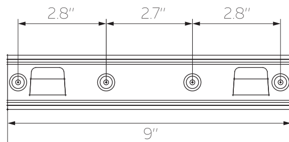
LOWER BRACKET
