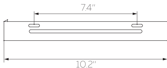
UPPER BRACKET
