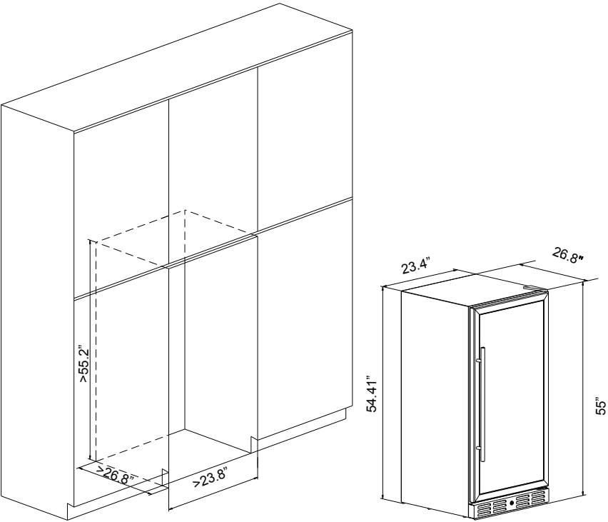
⦿ Installation Drawing
