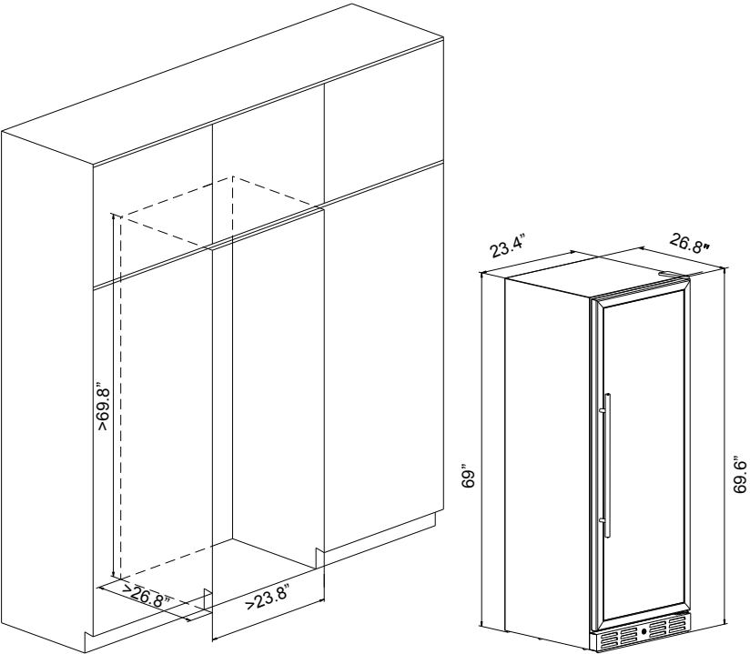
⦿ Installation Drawing
