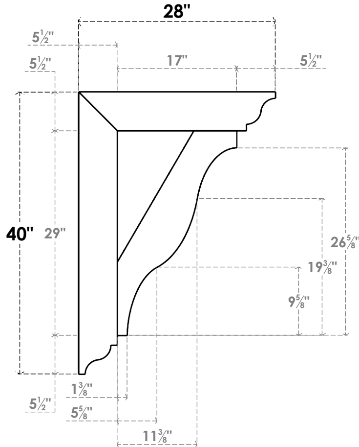
SIDE PROFILE
