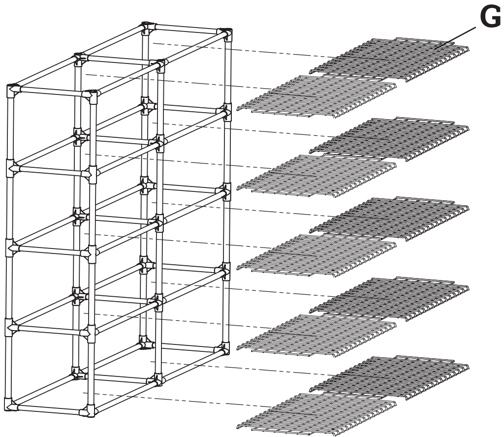
Place the mesh layers
