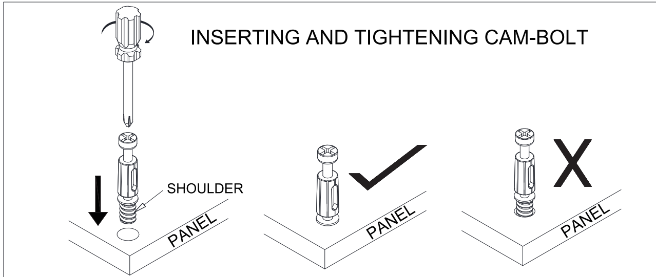
CAM-BOLT
