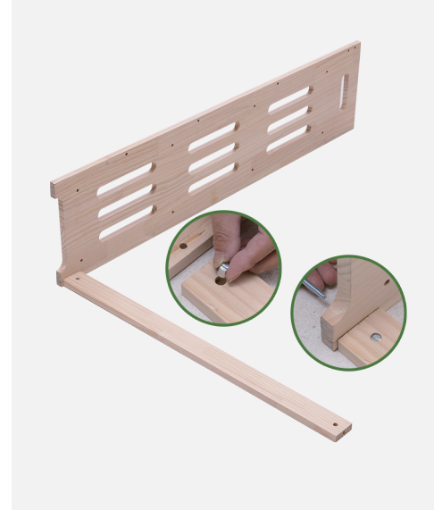
① Position and secure Back Slat (d) on Frame (b) with Screws (f).
