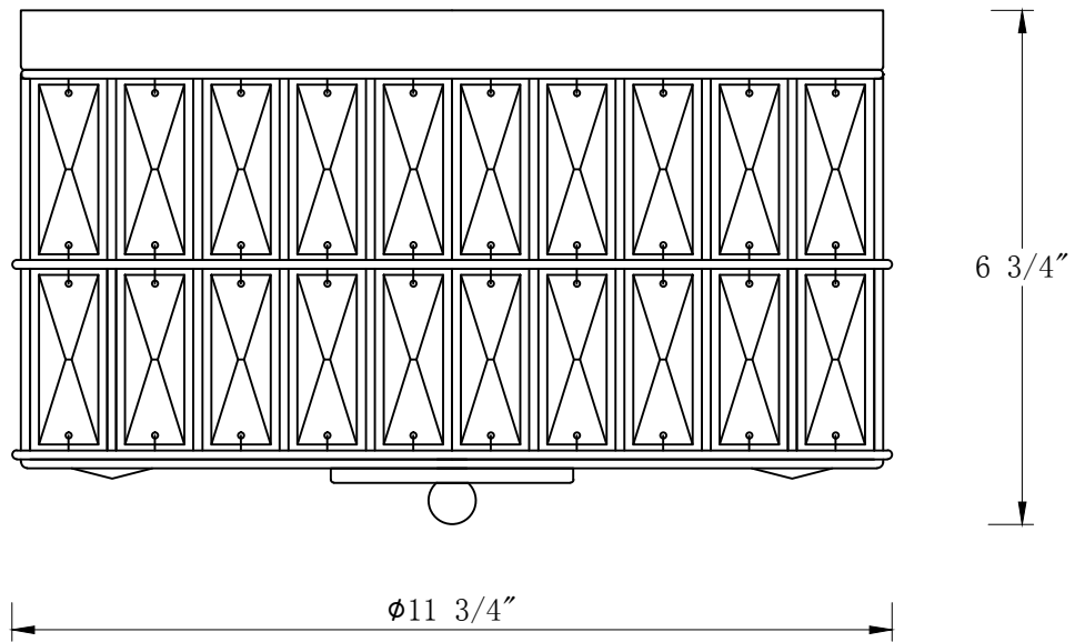
FRONT VIEW
