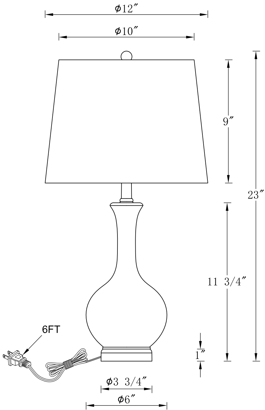
FRONT VIEW
