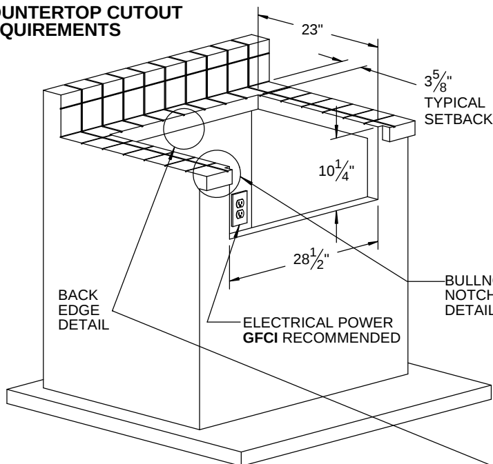
TYPICAL ALXE-30 / 30SZ INSTALLATION
