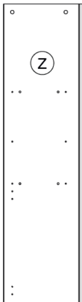
FI9090 1250x330x30mm
