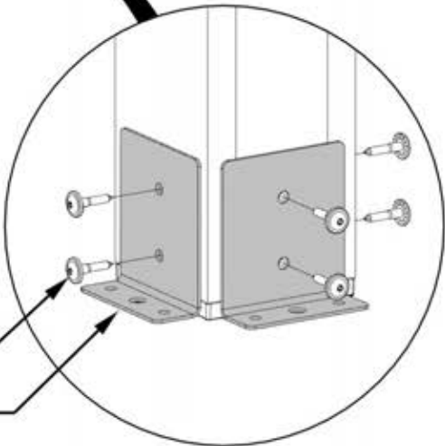
977 (x12) POST ANCHORING PLATE
