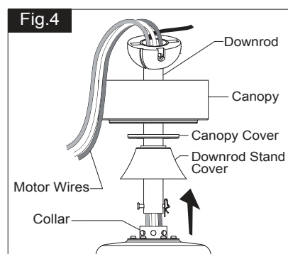
Slide canopy, canopy cover and downrod stand cover onto downrod, as shown; then thread motor wires through downrod.
