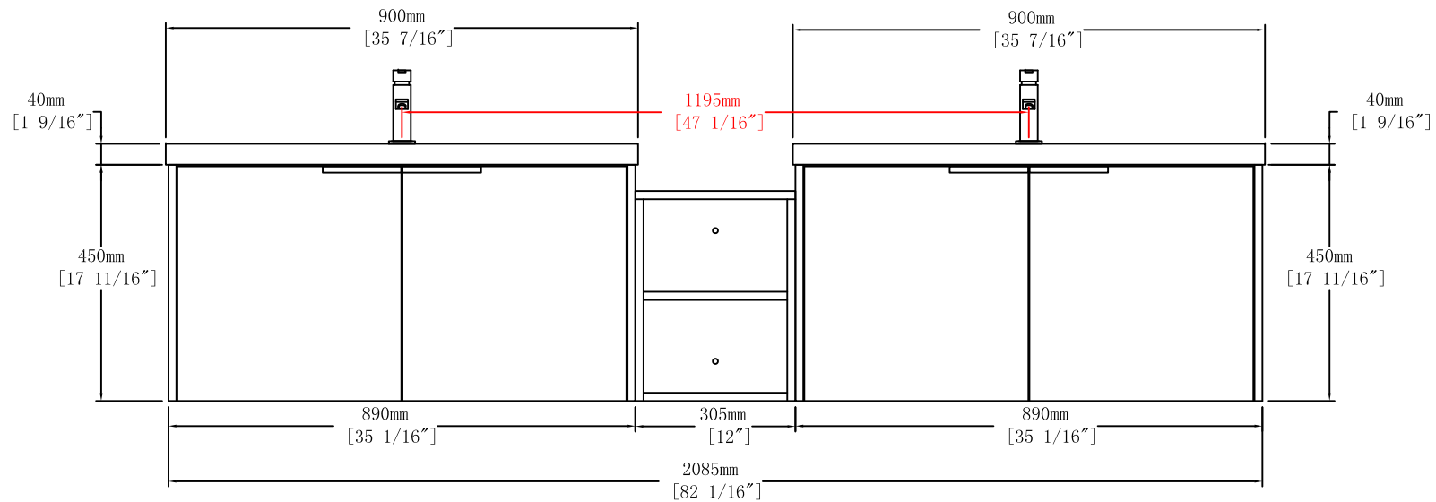
Front View
