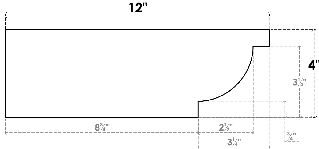
SIDE PROFILE
