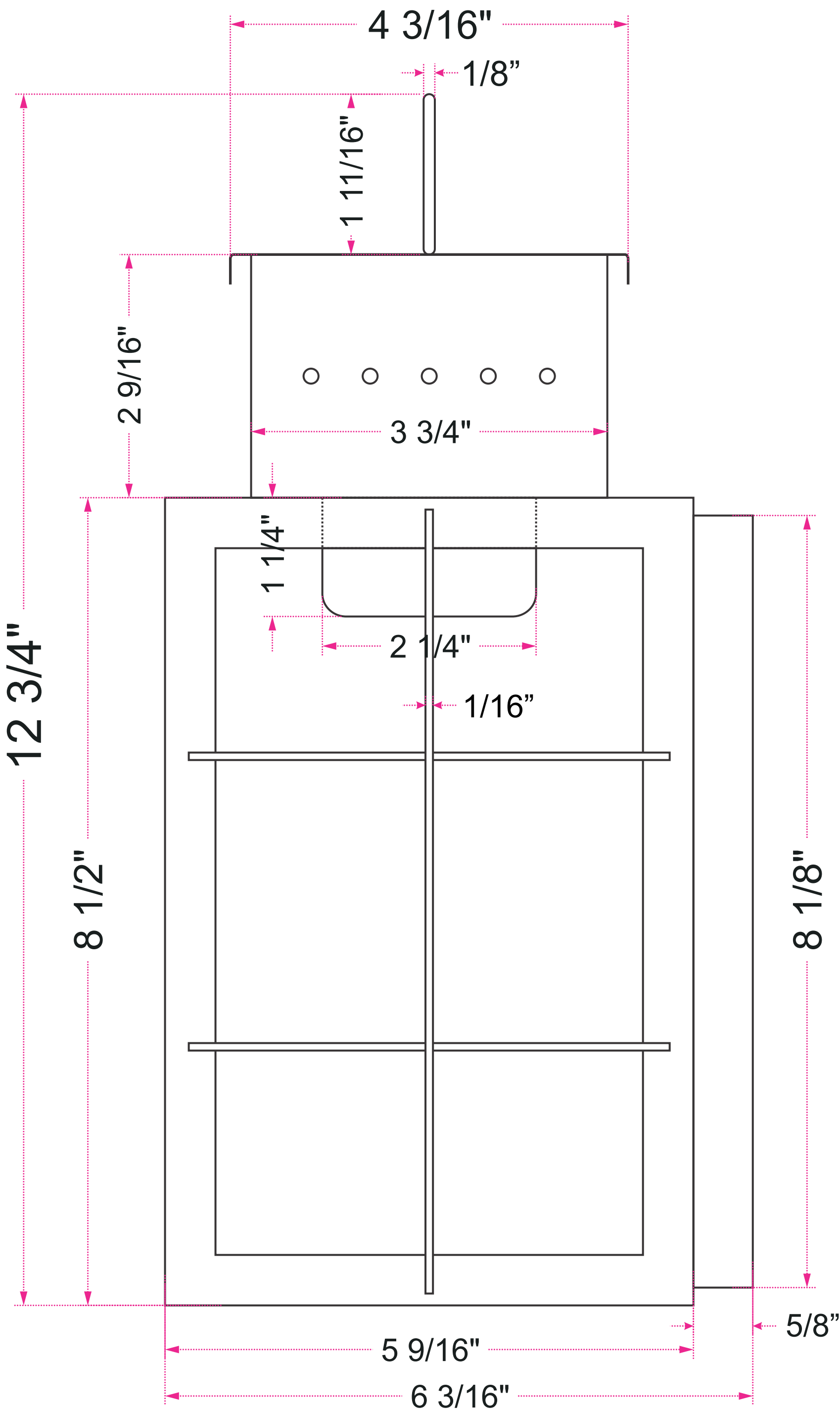
Side View
