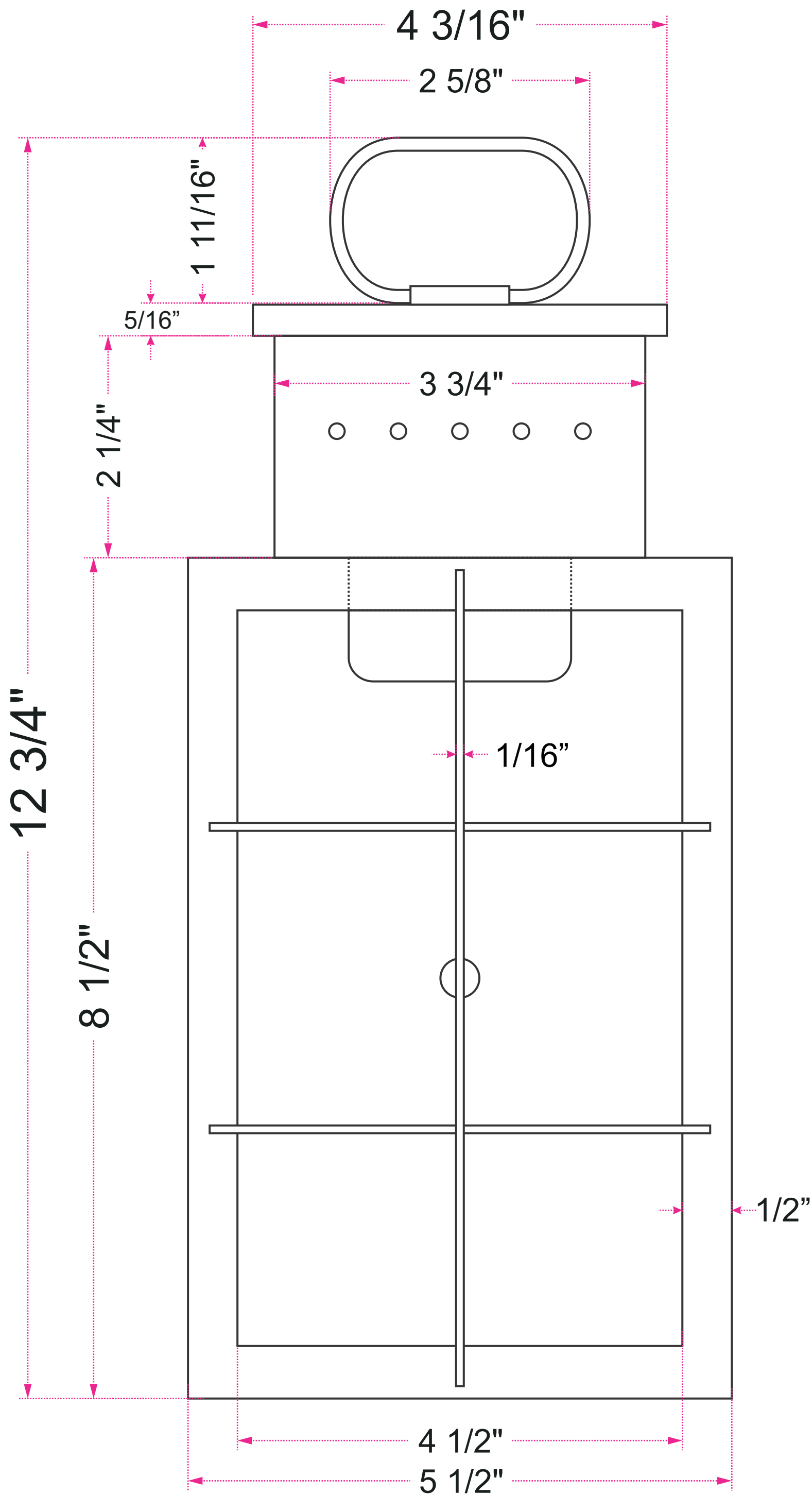
Front View
