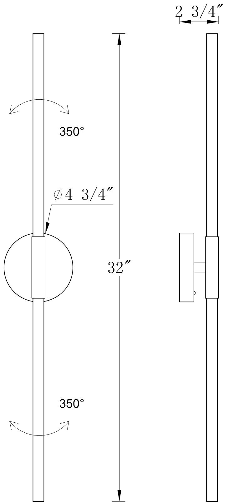
FRONT VIEW
