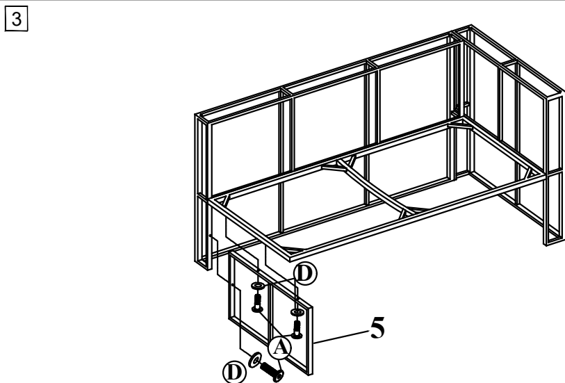
Step 3 Connect part from Step 2 & Front Right Frame (5) tighten Bolt (A) with Allen key (E)
