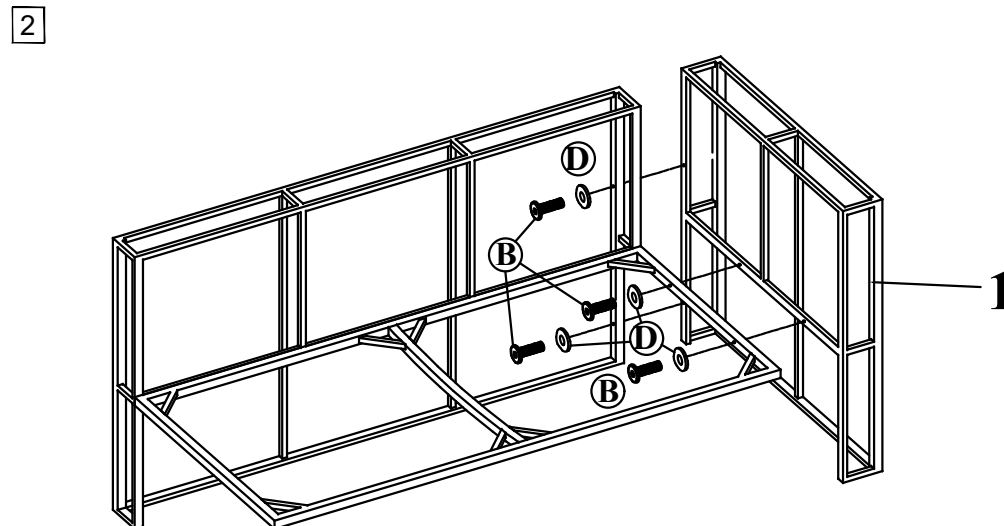
Step 2 Connect part from Step 1 & Left Frame (1) tighten Bolt (B) with Allen key (E)
