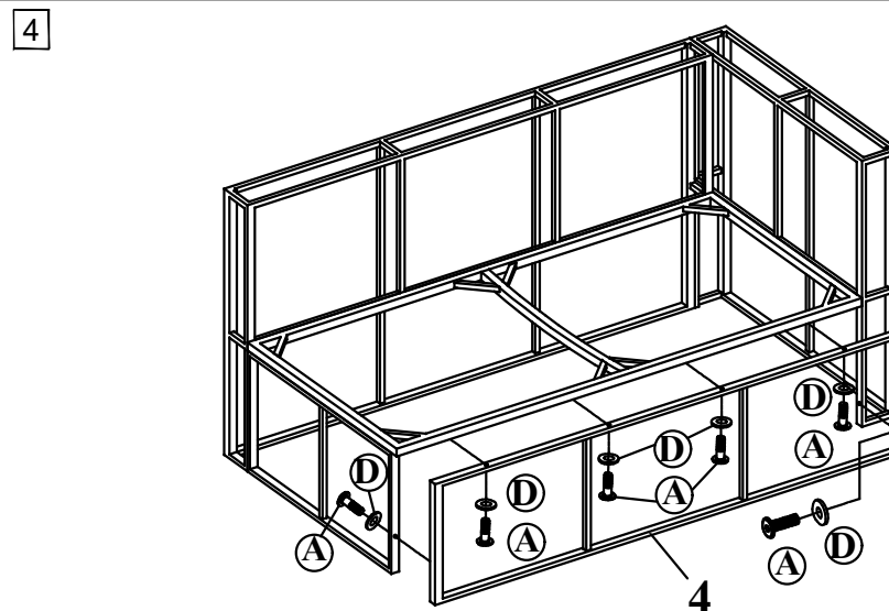
Step 4 Connect part from Step 3 & Bench Front Frame (4) tighten Bolt (A) with Allen key (E)
