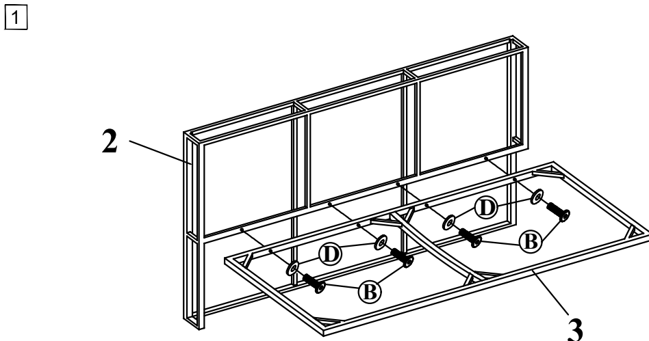
Step 1 Connect Bench Back Frame (2) & Bench Seat Frame (3) & tighten Bolt (B) with Allen key (E)
