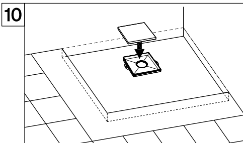
10. Cover the drain opening to prevent any debris from going into the drain.
