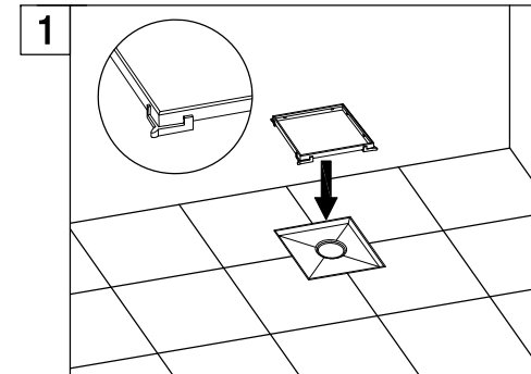
1. Fasten the 4 tray support clips by snapping them into the sides of the tile insert tray.
