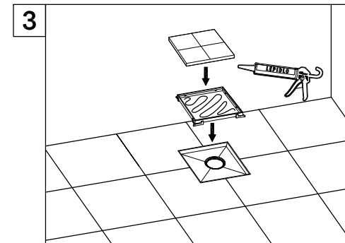
3. Apply an even coat of tile adhesive to the back of the tile and press into place, set the tile so that it sits 1mm above the rim of the tray, this will prevent any water from pooling on top of the tile-insert.
