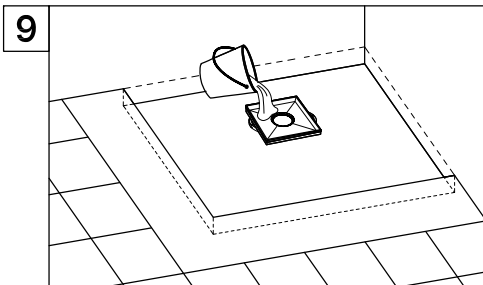
9. Test that all connections are watertight by pouring some water and checking for leaks.
