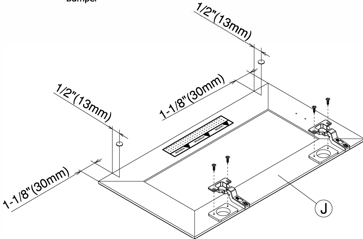
Bumper
