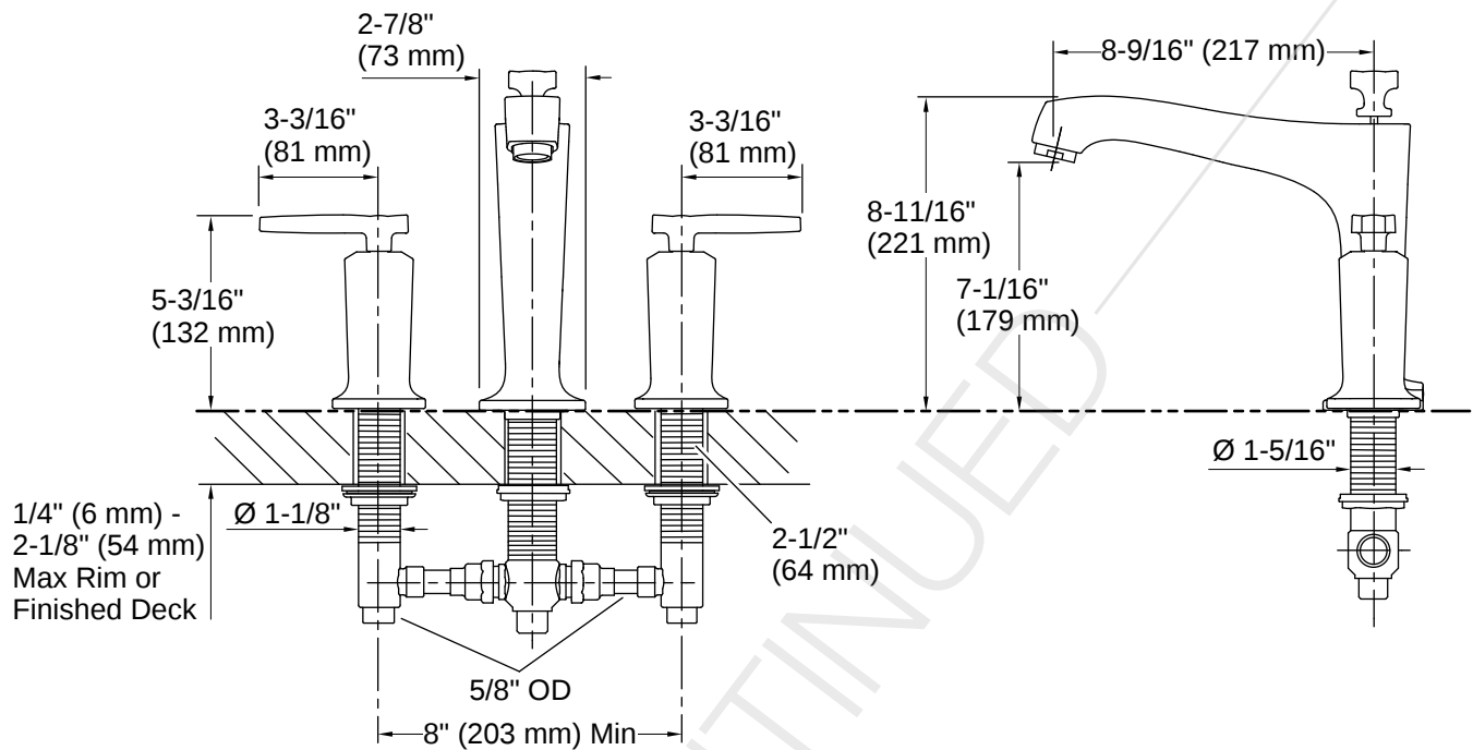
Rim or Finished Deck Mount Installation
