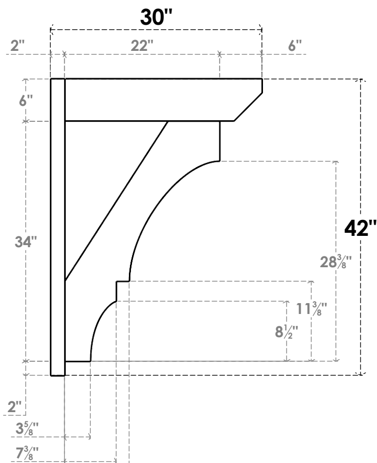
SIDE PROFILE
