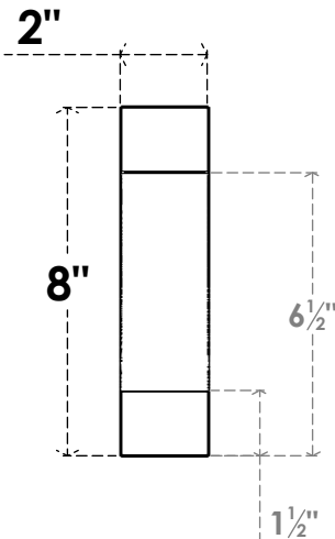
FRONT PROFILE
