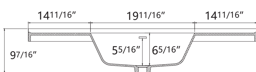
Front View
