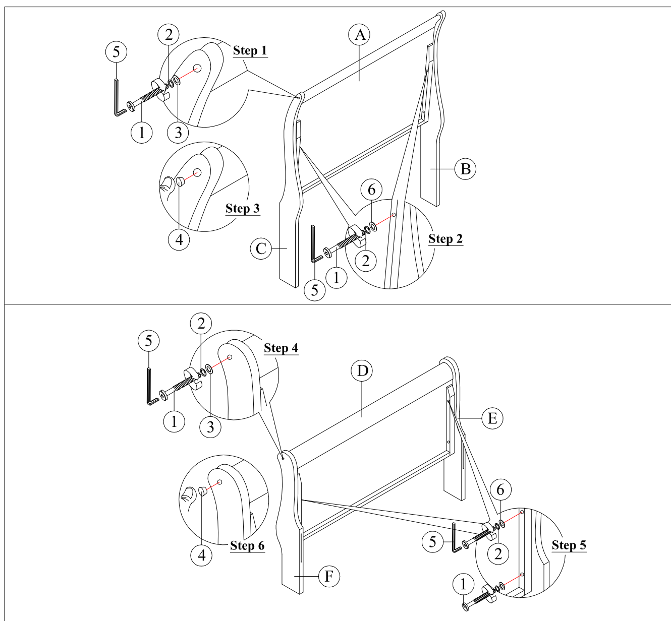
COMPLETED TWIN BED ASSEMBLY
