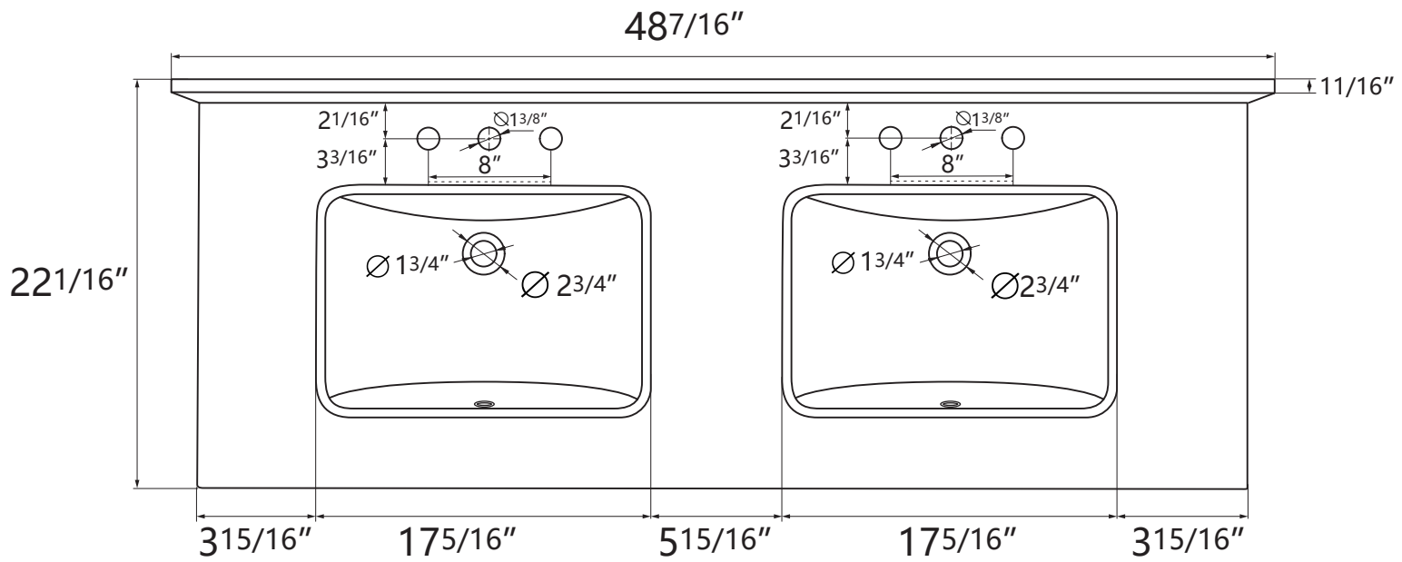
Top View
