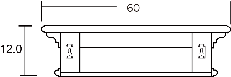
BACK VIEW
