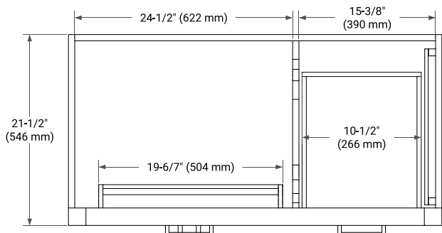
PLAN VIEW
