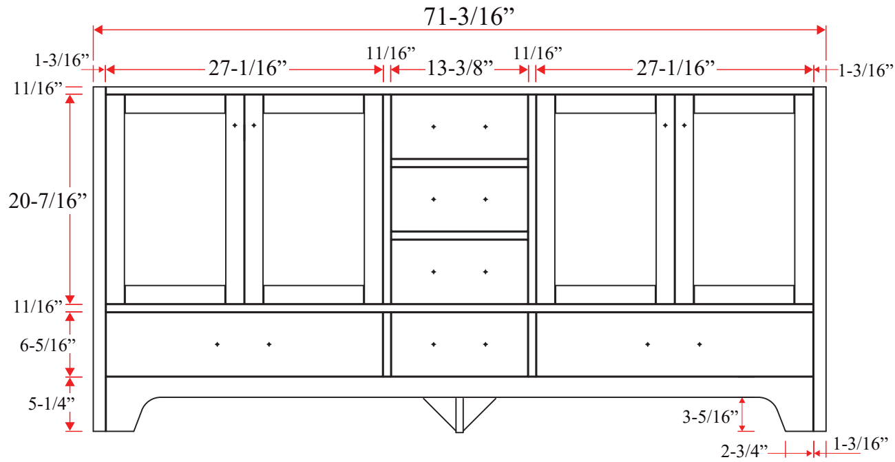
FRONT VIEW
