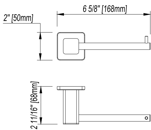
ROLL HOLDER
