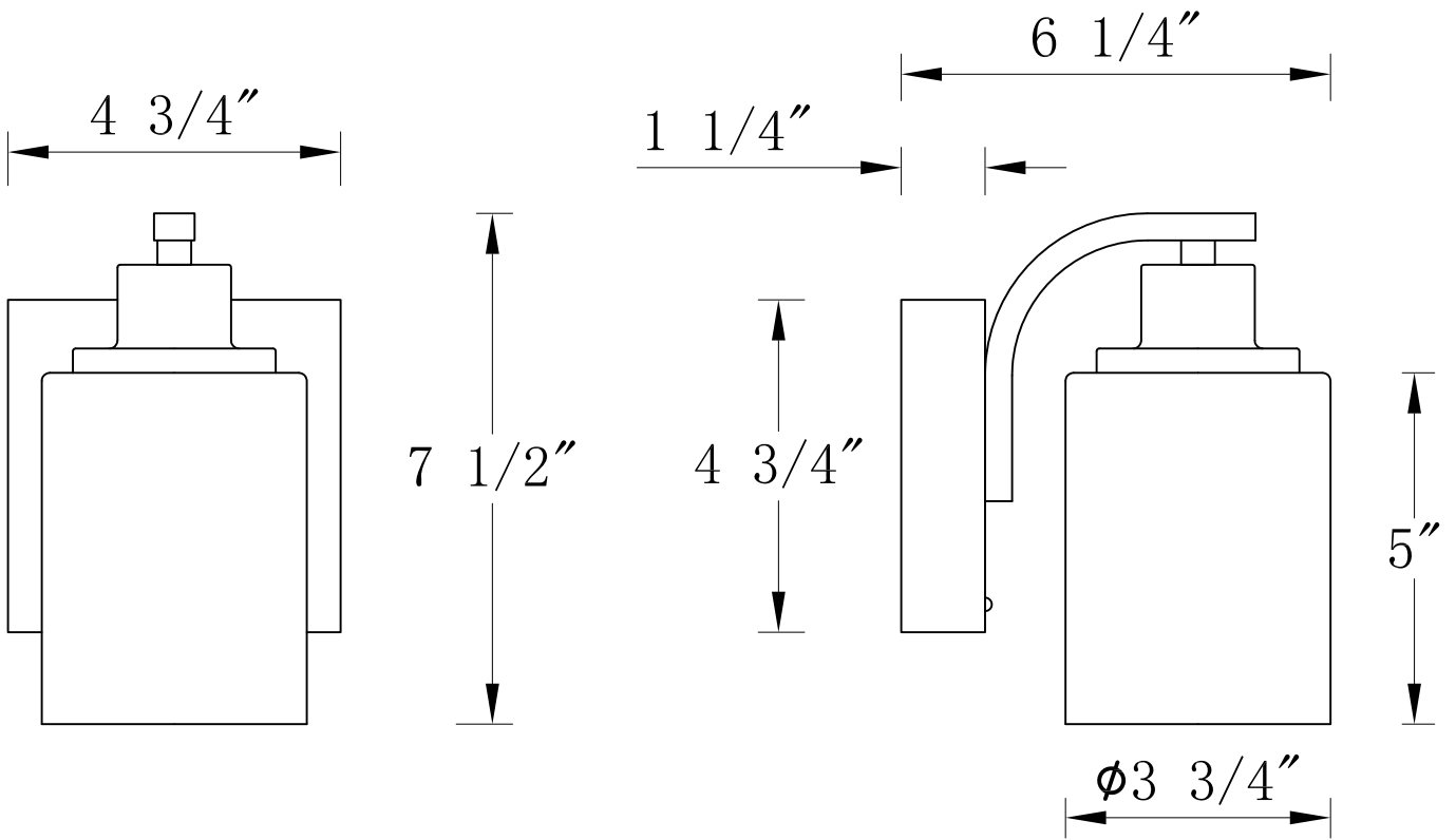
FRONT VIEW
