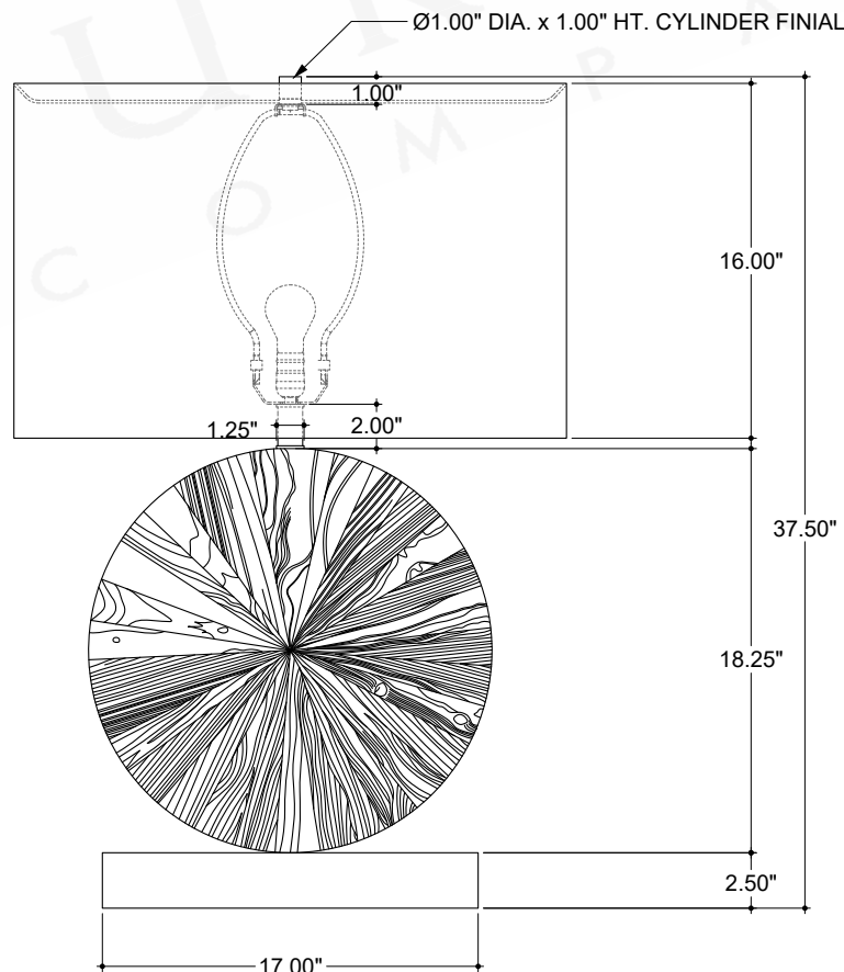
FRONT VIEW
