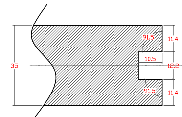
STILE SECTION
