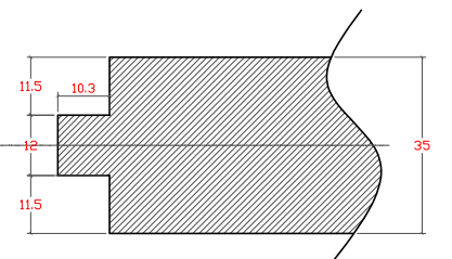
TOP/BOTTOM RAIL SECTION
