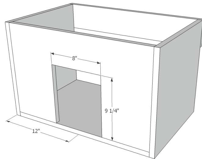
BACK DETAIL
