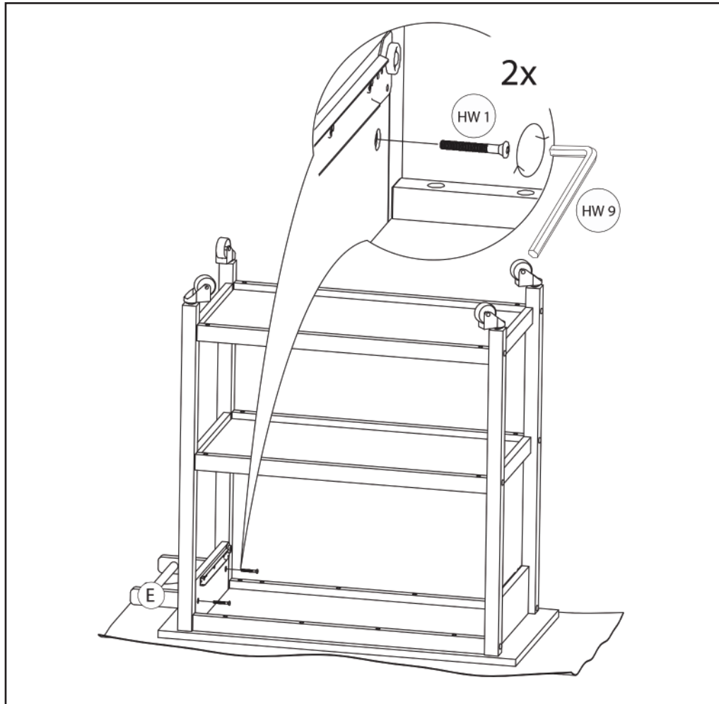
Step 5 : Assemble the handle bar.
