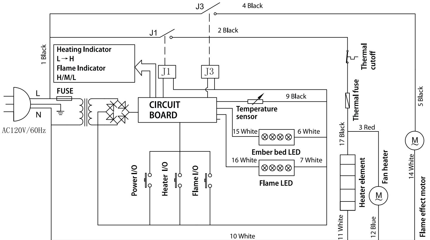
CIRCUIT DIAGRAM
