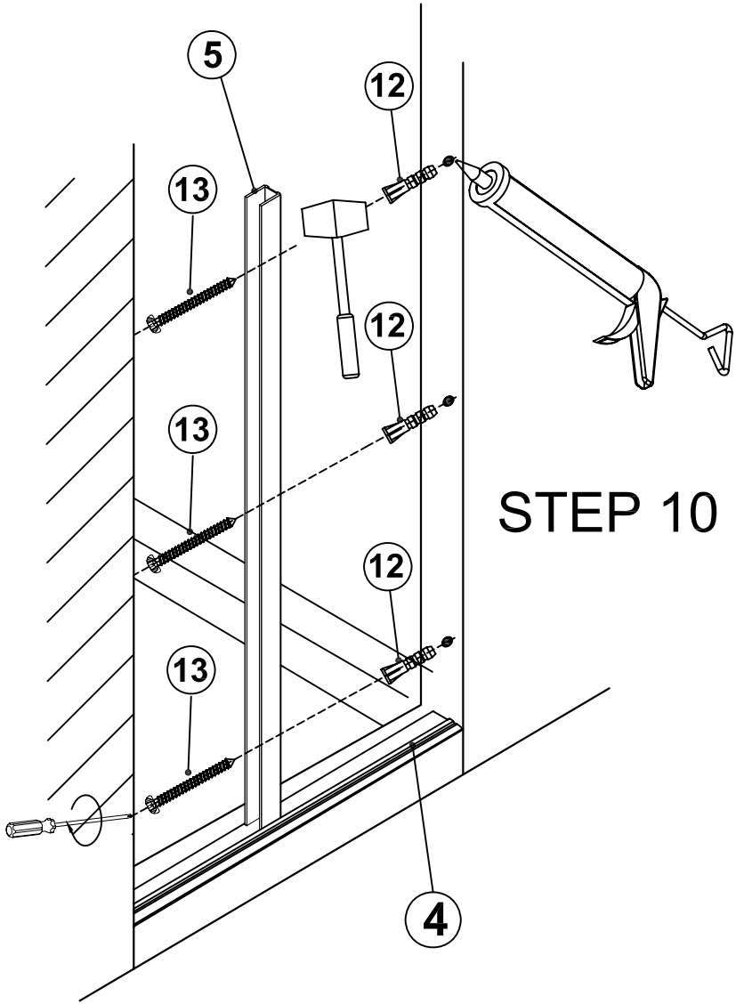
⑬ SCREW 1 1/2"
