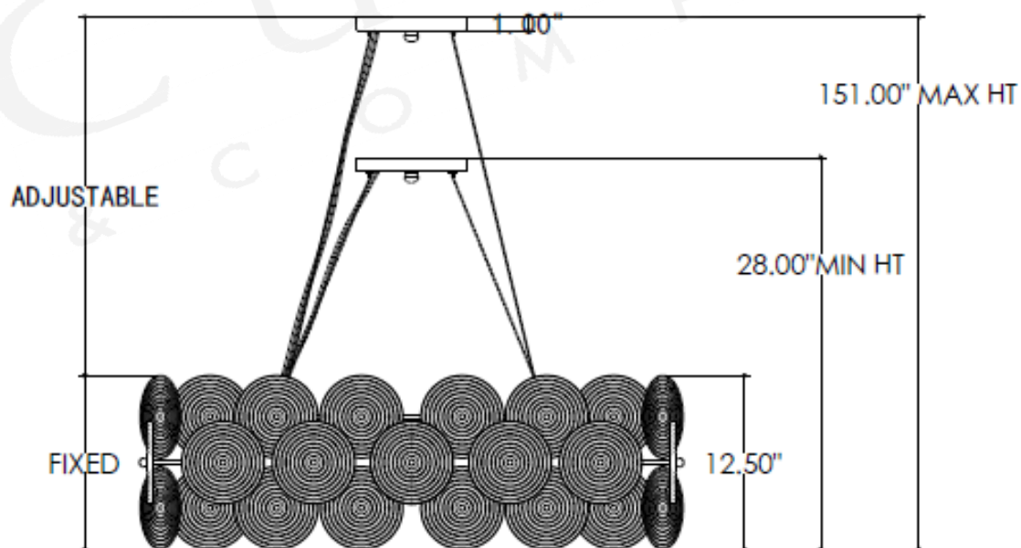
FRONT VIEW
