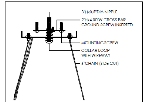
CANOPY DETAILS
