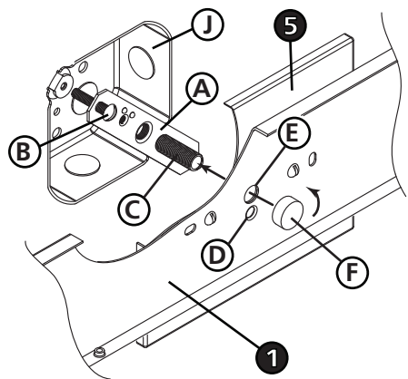
DRAWING 1 - MOUNTING
