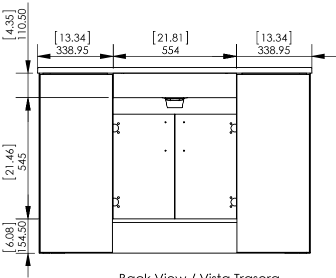
Back View / Vista Trasera
