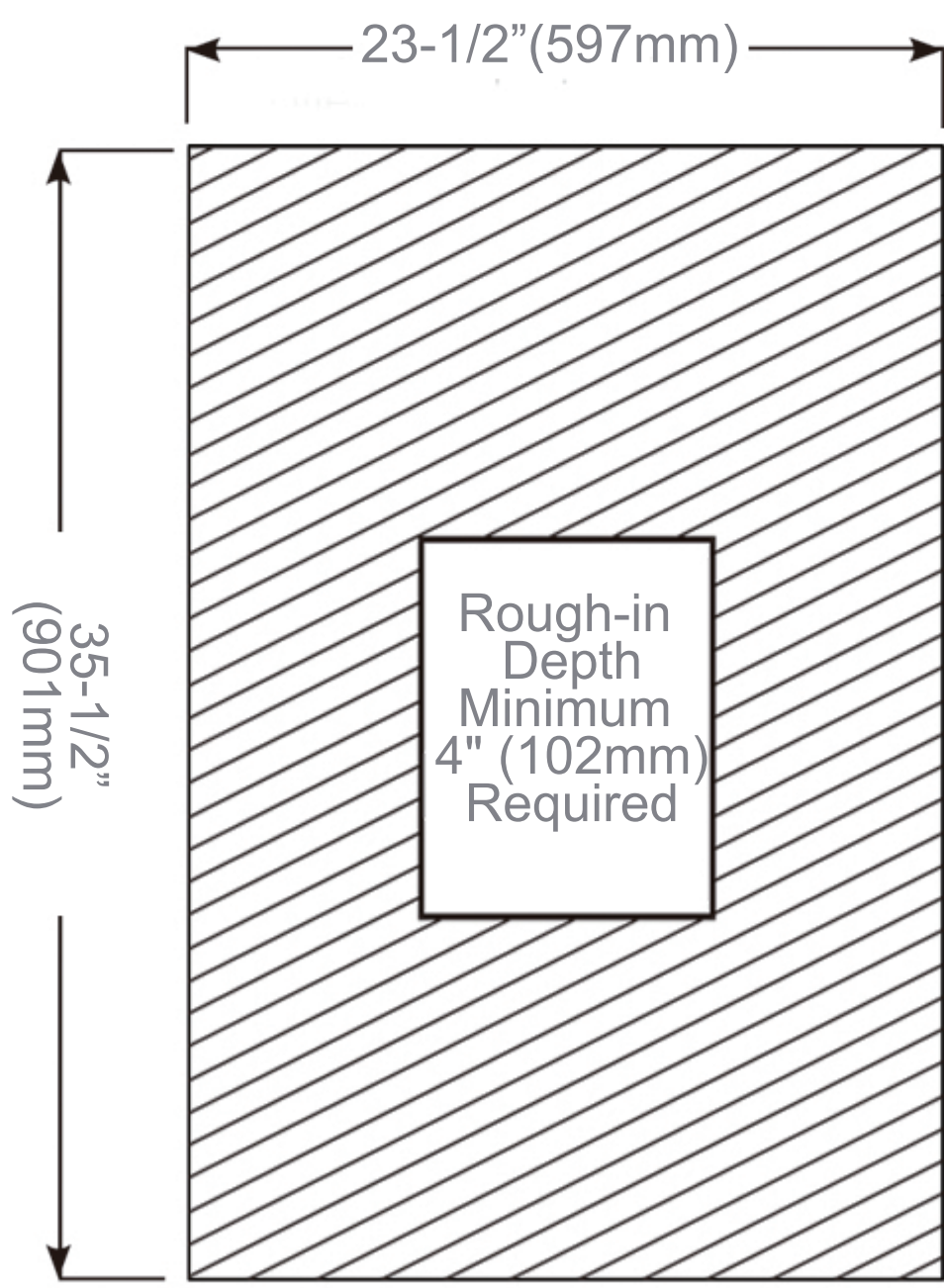
Rough-in Dimensions
