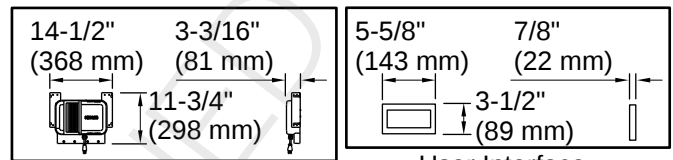
Control Amplifier
