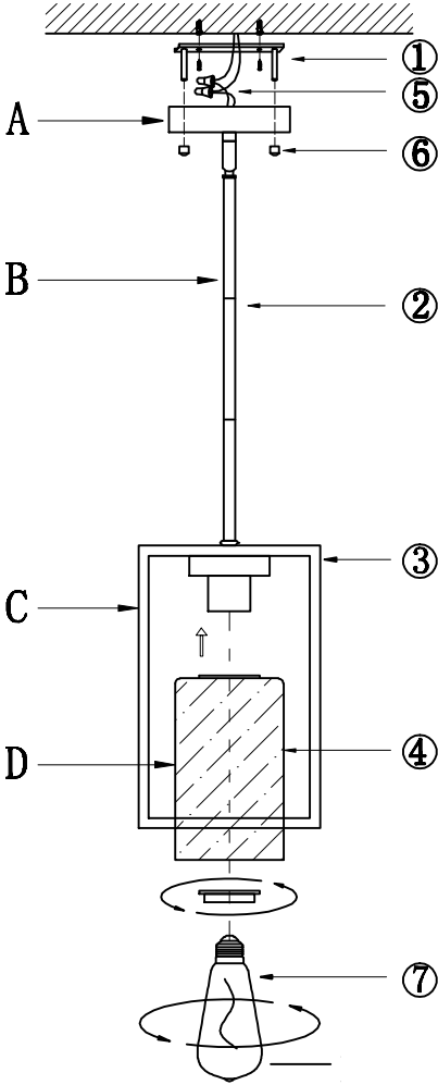
Installation sequence diagram
