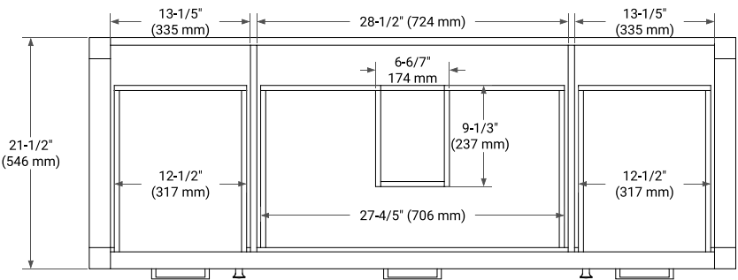
PLAN VIEW
