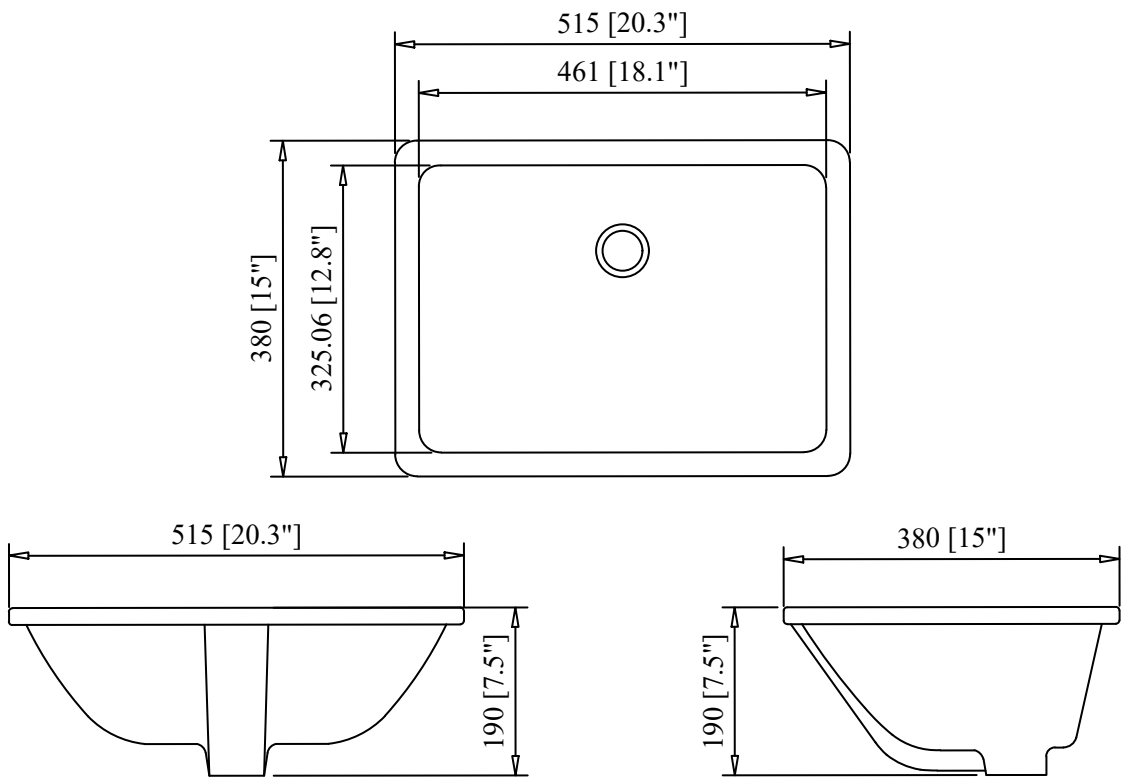
Undermount Sink
