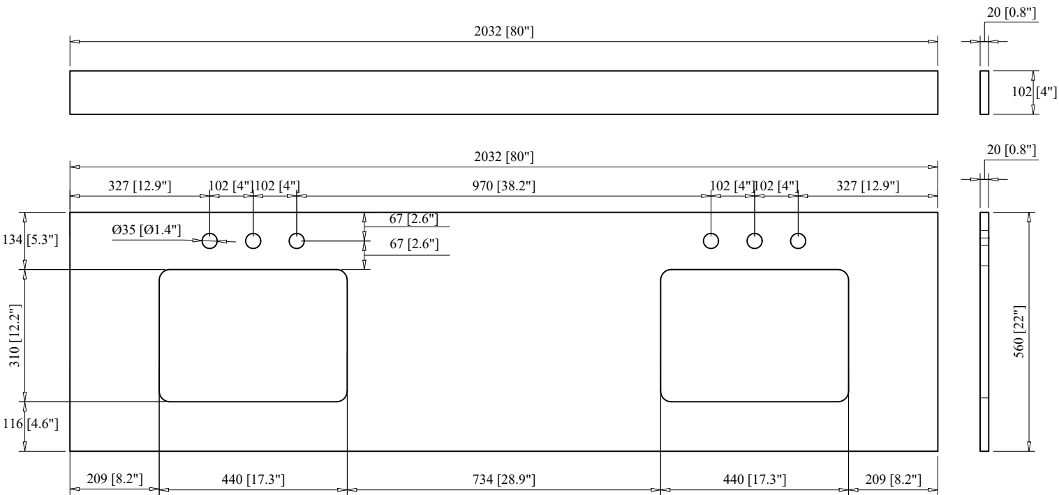
VanityTop
